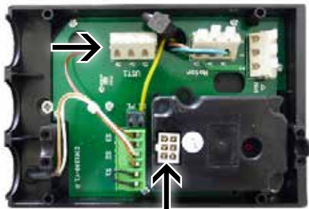
Six-pole plug Control connection cable
