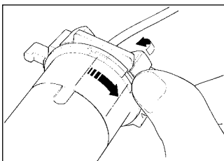
Turn the ring nut until the bevel coincides with one of the connecting teeth, and then disconnect.
